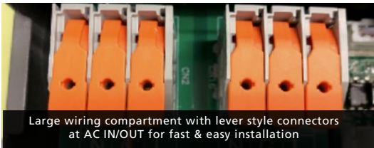
Hardwire or plug directly into the optional 20A GFCI receptacle
