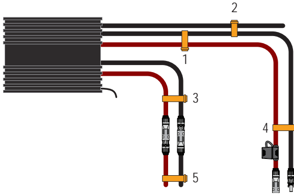
Figure 7 Strain-relief points
