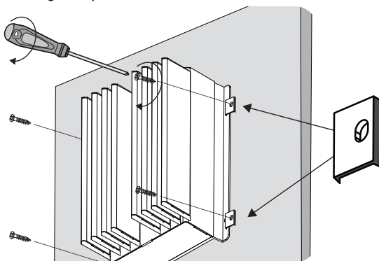
Figure 6 Flange adapter
