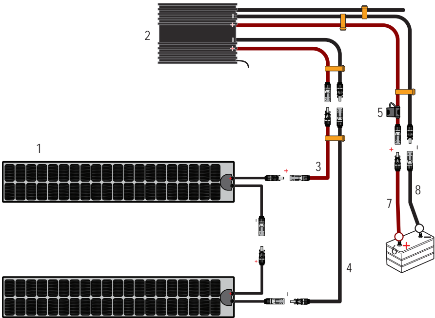
Figure 1 Complete cable schematic of a 2-solar panel power system
